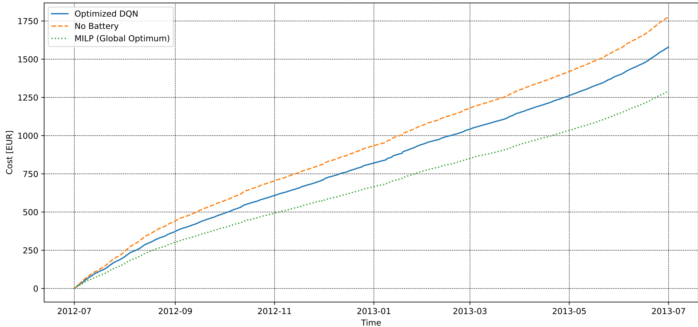
User 137 - Extended Convergence - Electricity Cost [DQN vs MILP]
